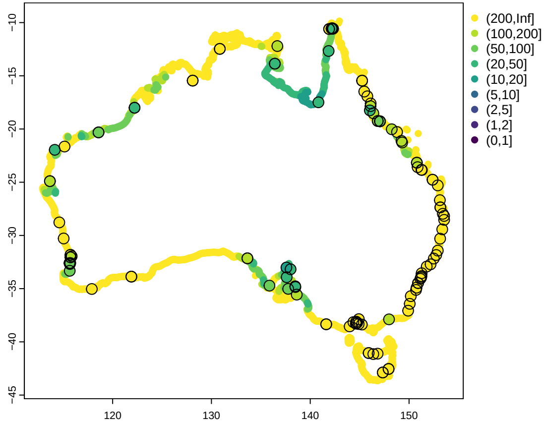
Extreme SWL multiplication factor for 0.54m of SLR
