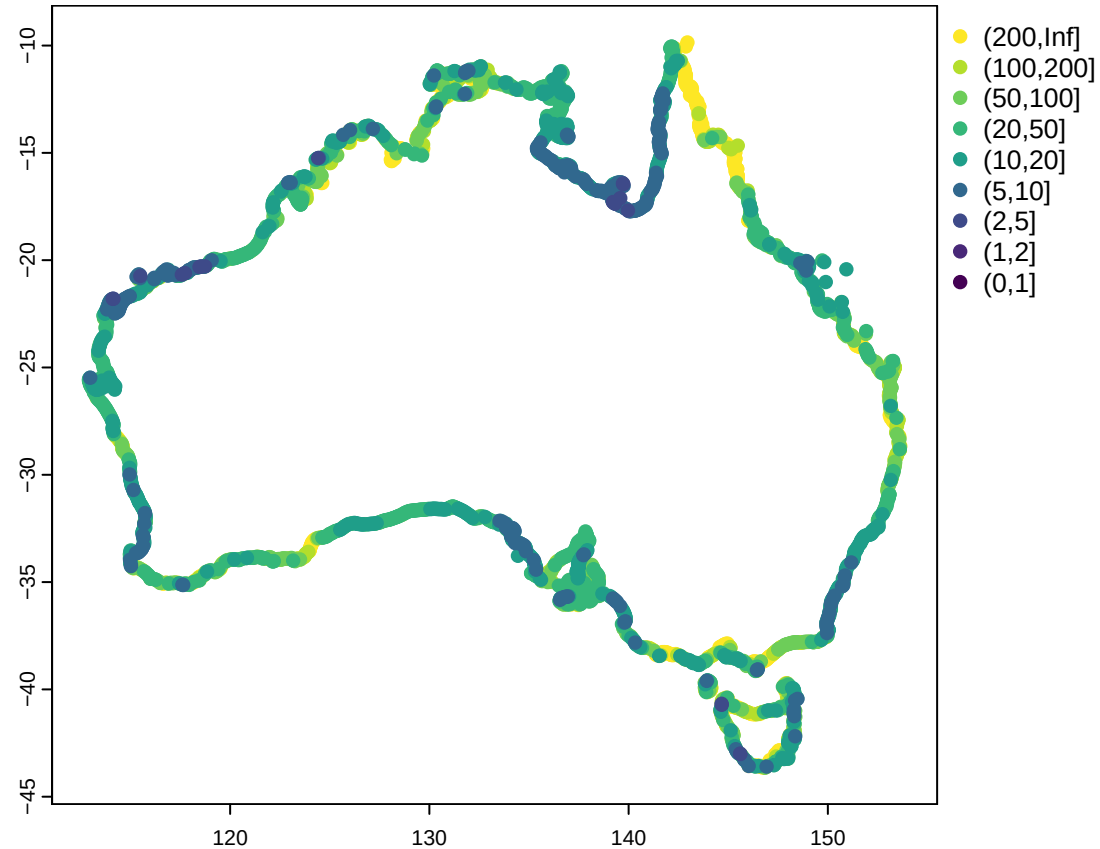
Extreme MTWL multiplication factor for 0.54m of SLR
