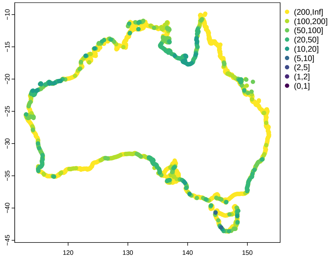
Extreme MTWL multiplication factor for 0.9m of SLR
