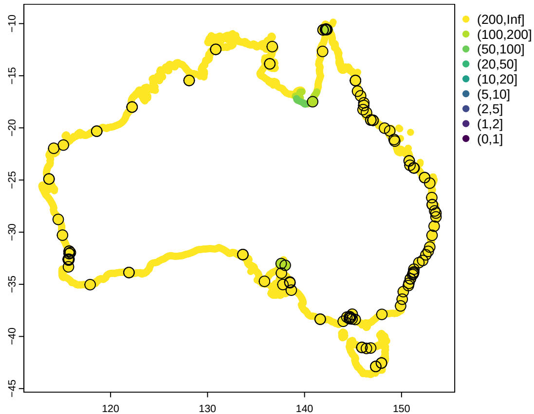
Extreme SWL multiplication factor for 0.94m of SLR
