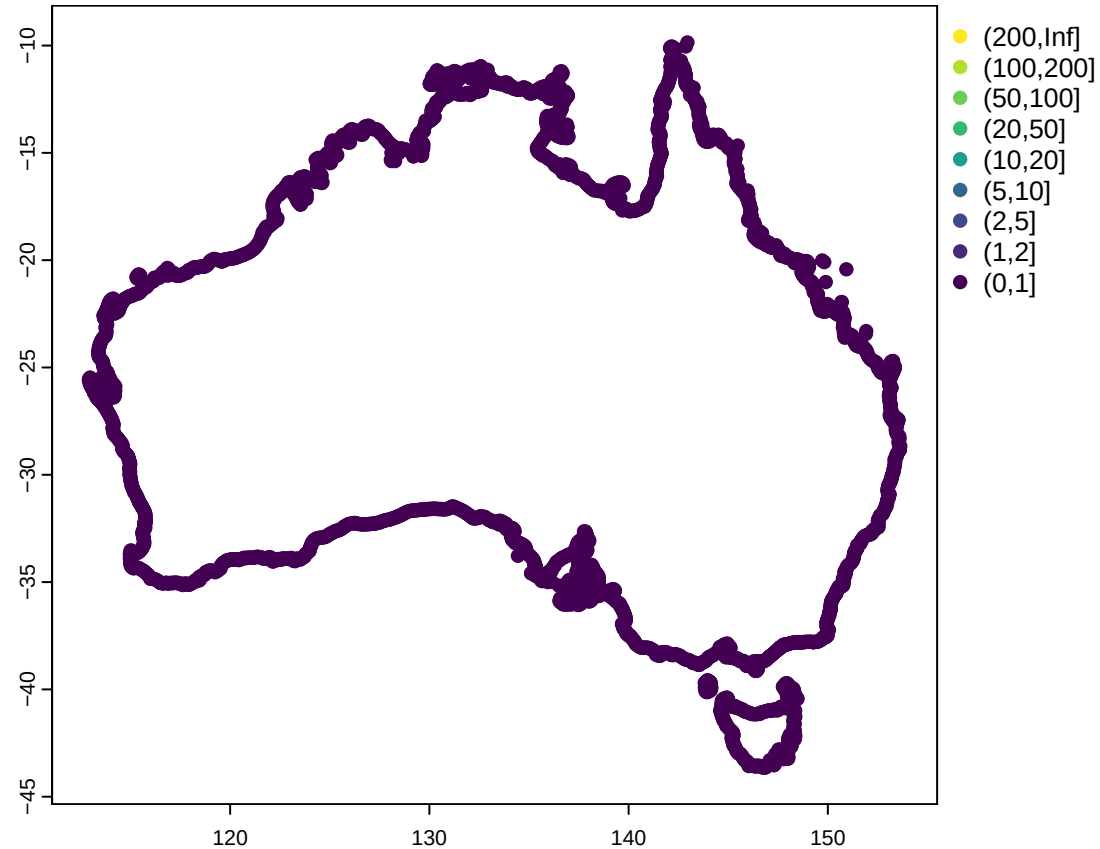
Extreme MTWL multiplication factor for 0m of SLR
