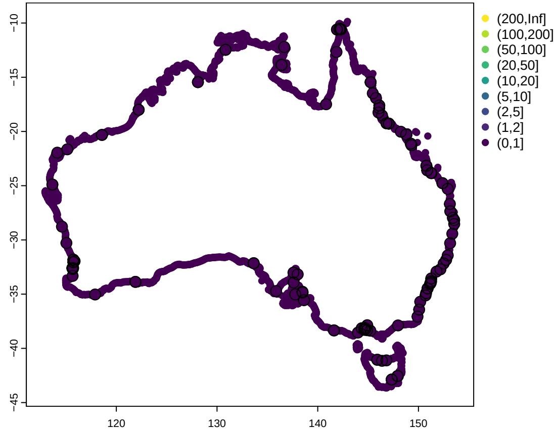
Extreme SWL multiplication factor for 0m of SLR
