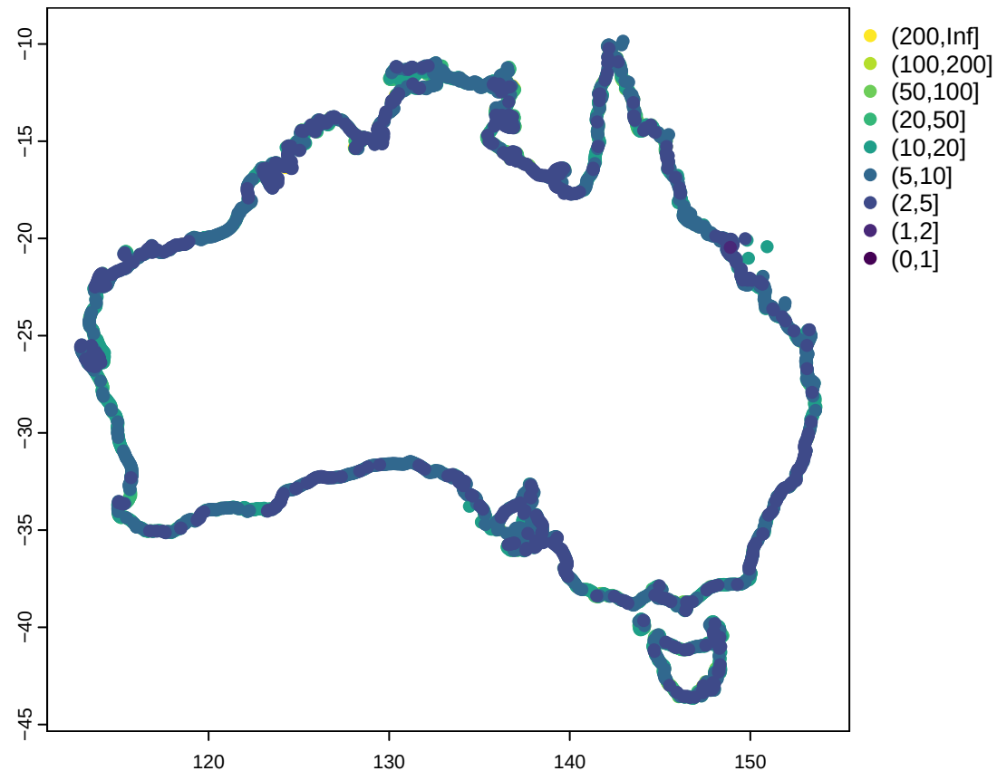
Extreme MTWL multiplication factor for 0.32m of SLR
