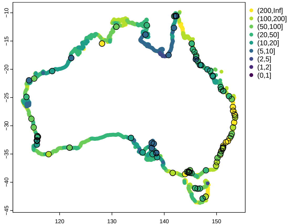
Extreme SWL multiplication factor for 0.32m of SLR
