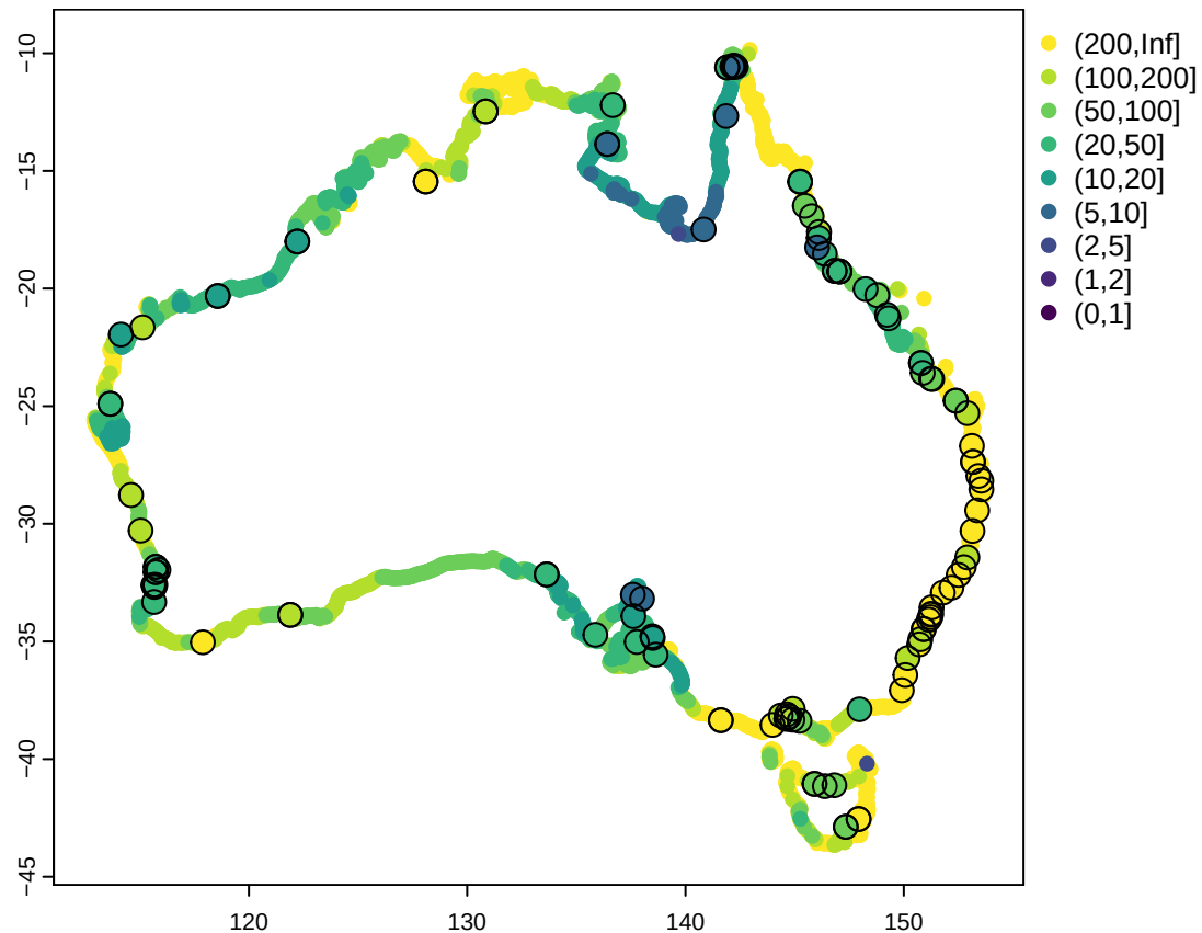
Extreme SWL multiplication factor for 0.38m of SLR
