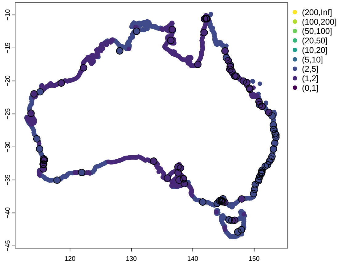
Extreme SWL multiplication factor for 0.06m of SLR
