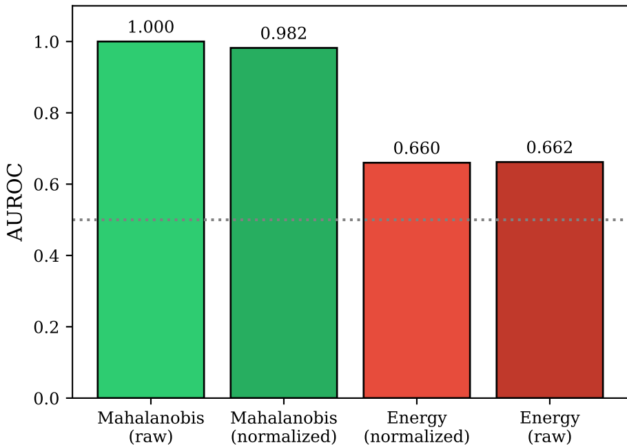
Superclass OOD Detection Performance (LOSO Cross-Validation)
