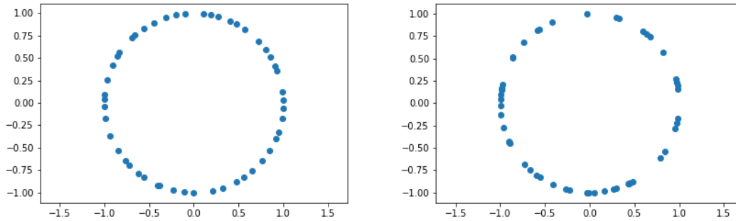
(a) A sample from the probability distribution |\Psi_0^A(z_1, \dots, z_N)|^2 for 50 particles. (b) Uniformly distributed points on the circle described by |\Psi_0^S(x_1, x_2, \dots, x_N)|^2 . The particle positions are uncorrelated.
