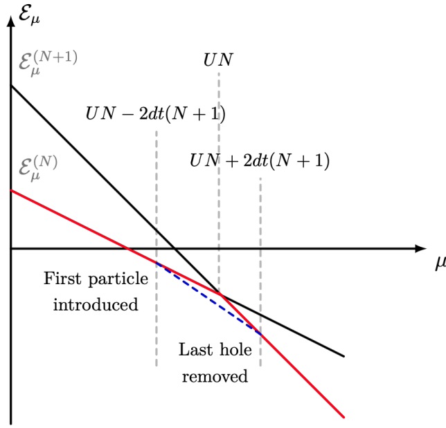
Figure 2.2: Comparing the energies of the Mott states with single particle or hole states. At t = 0 the red line is the absolute ground state. For nonzero t the dashed blue line corresponds to non-integer filling. Figure by William Royce.
