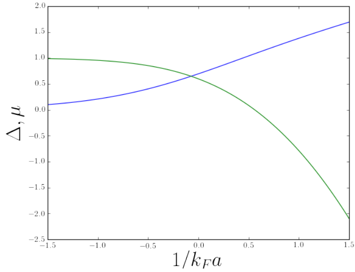
Figure 2.2: Variation of gap and chemical potential accross the BCS (left, weak attraction) to BEC (right, strong attraction).
