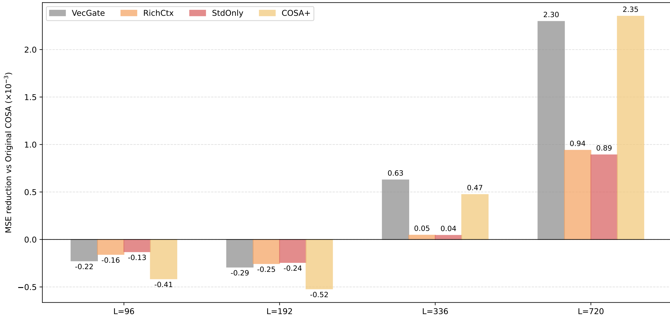
ETTh1 / DLinear Ablation: Improvement Over Original COSA
