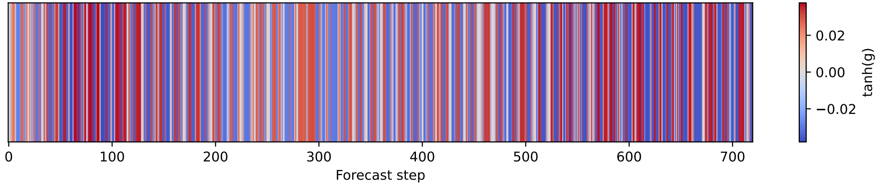
COSA+ Learned Vector Gate, ETTh1 / DLinear / L=720
