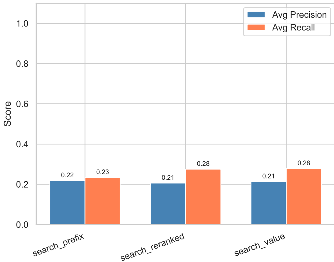
Search Tool Precision & Recall — Condition A
