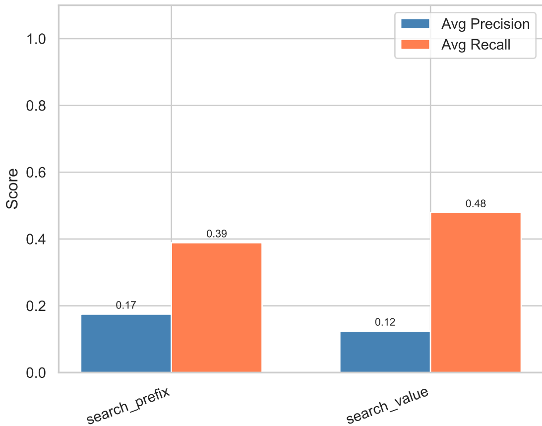
Search Tool Precision & Recall — Condition B
