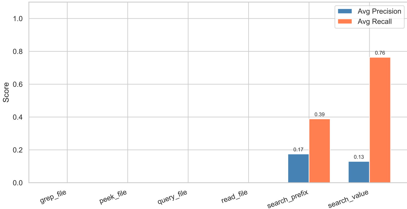
Search Tool Precision & Recall
