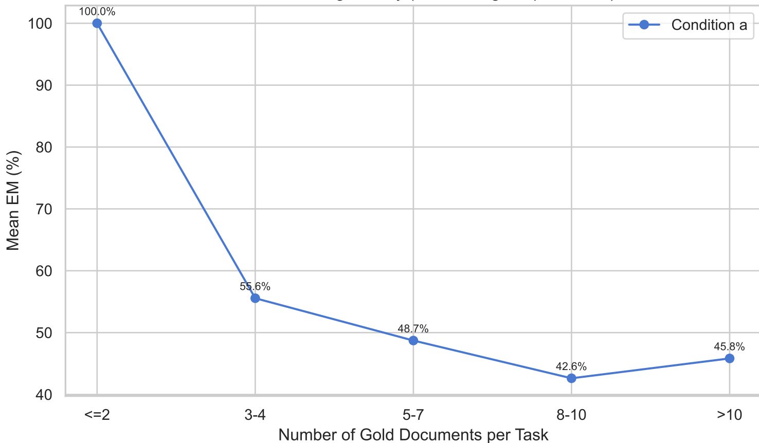
EM vs. Reasoning Density (LakeQA Fig 4 reproduction)
