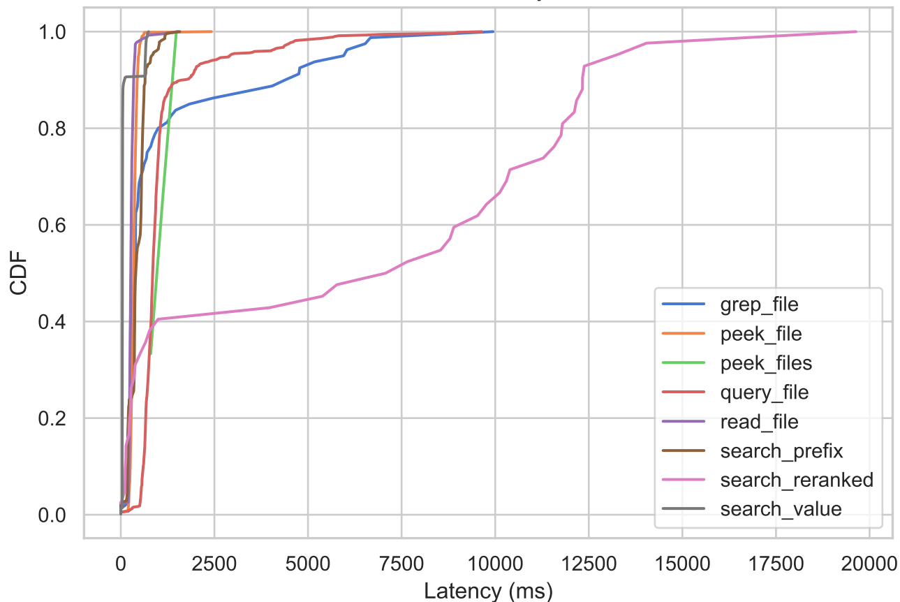
Tool Call Latency CDF
