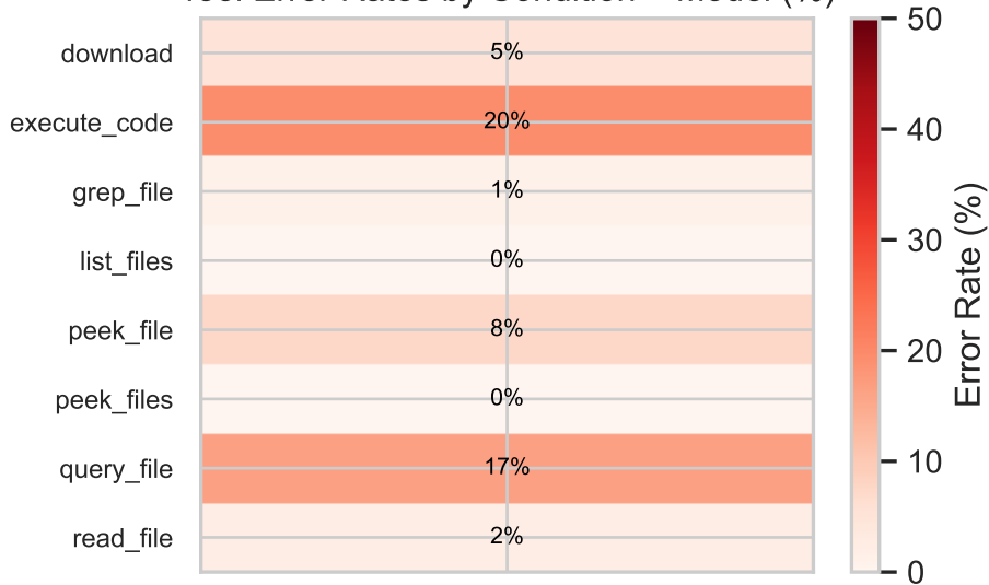
Tool Error Rates by Condition × Model (%)
