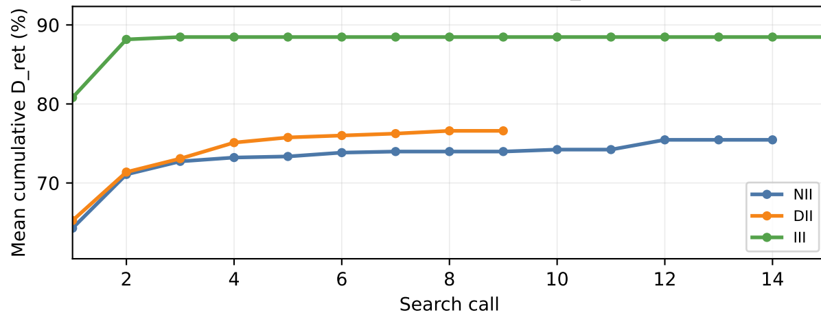
gpt-5.4-nano: Cumulative D_ret
