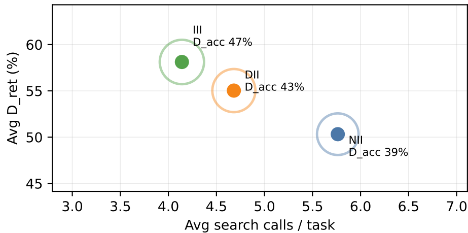
gpt-5.4-nano: Retrieval Efficiency
