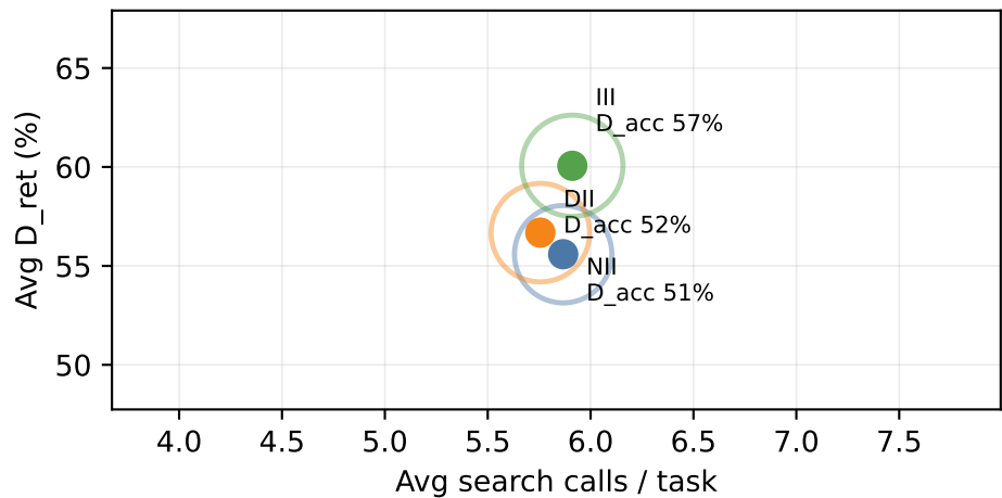
gpt-5-mini: Retrieval Efficiency
