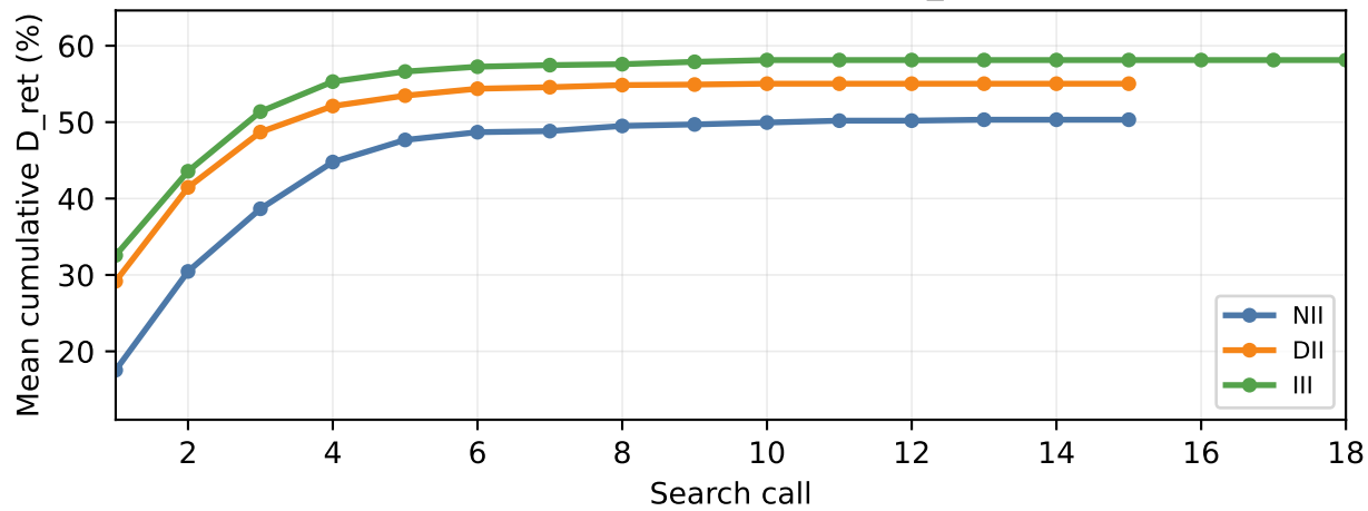
gpt-5.4-nano: Cumulative D_ret
