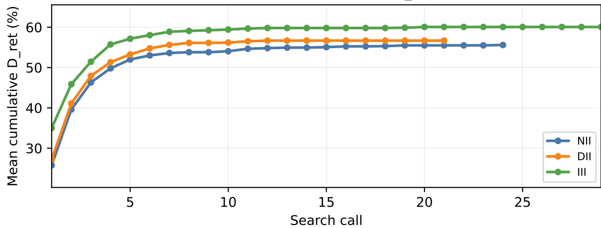
gpt-5-mini: Cumulative D_ret
