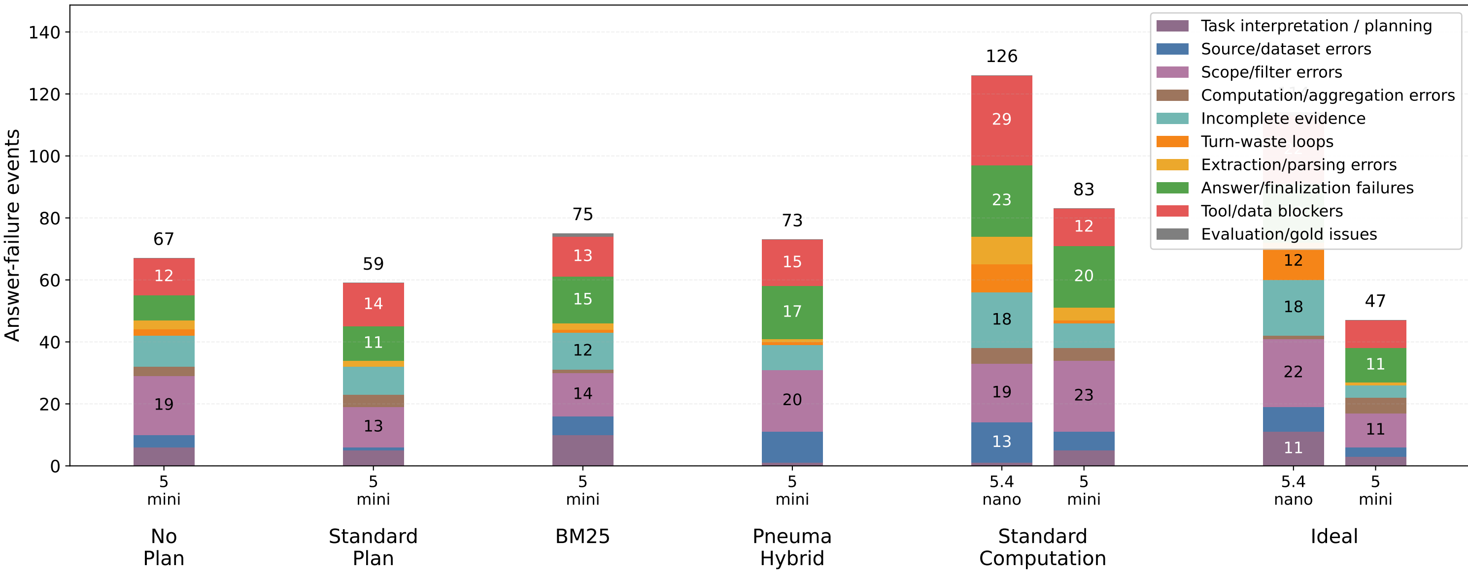
Answer-Failure Groups by SANA Condition and Model
