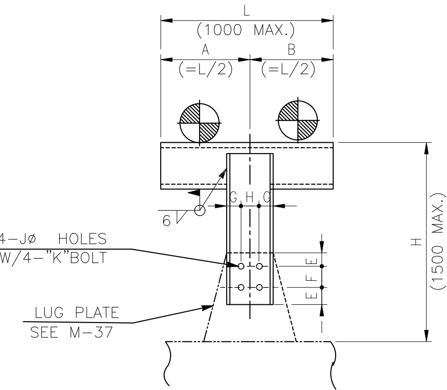
DIMENSIONS (mm)
