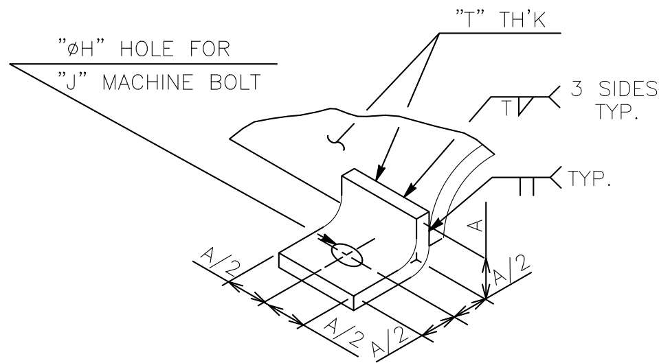
DETAIL "Z"
