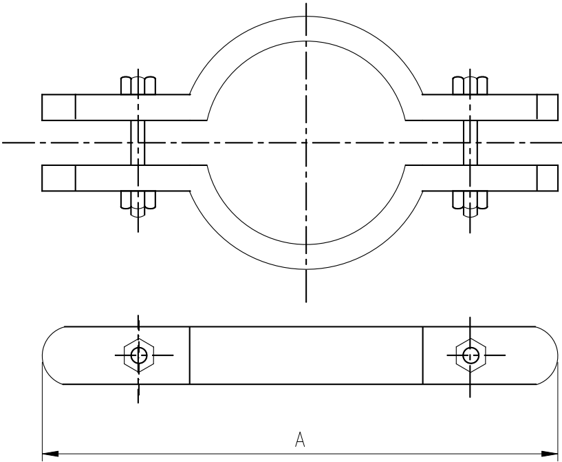
DIMENSION (mm)
