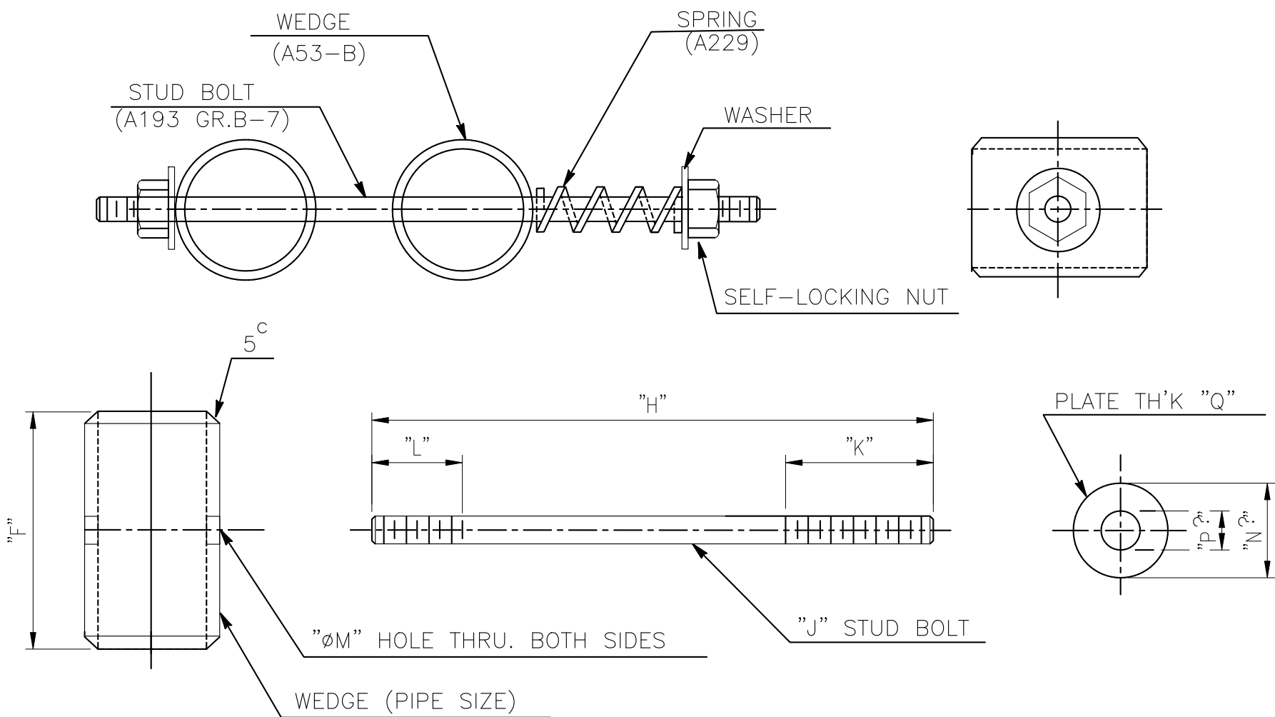
DIMENSIONS (mm)
