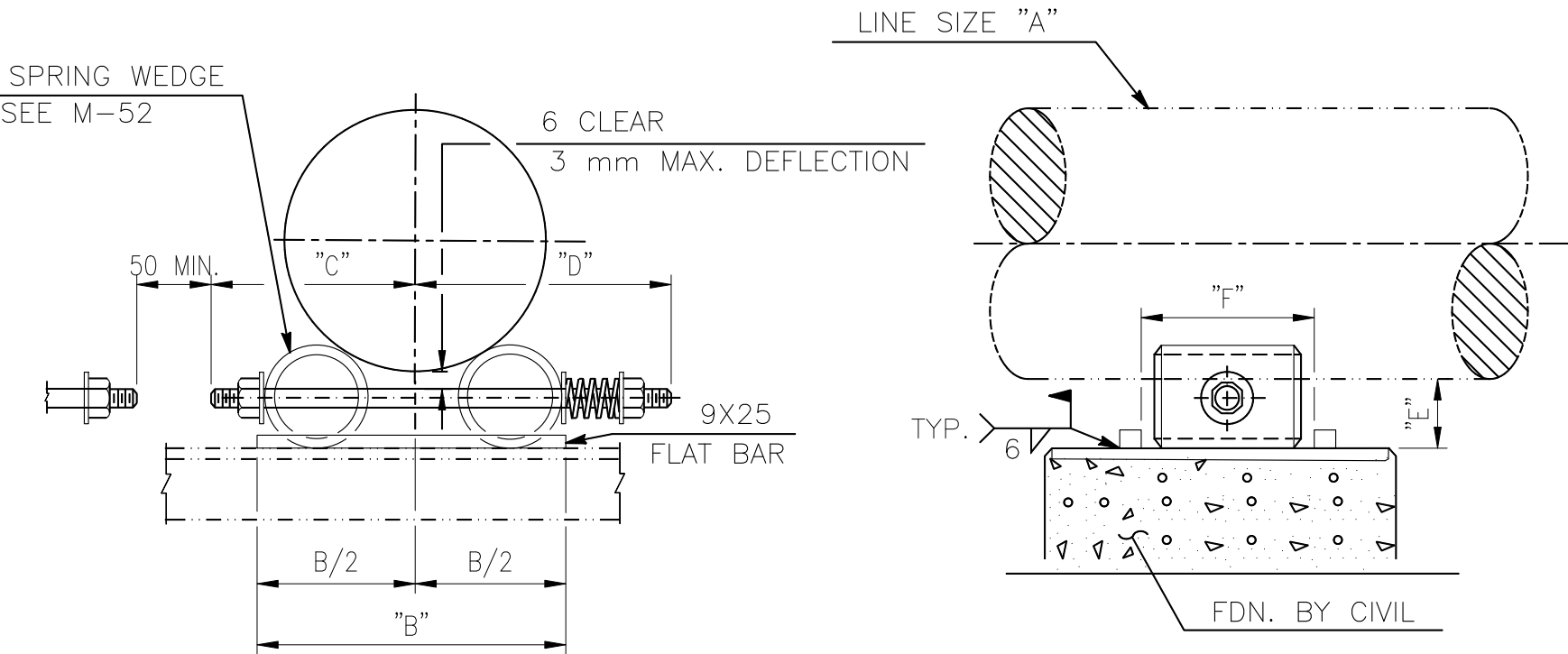
DIMENSIONS (mm)
