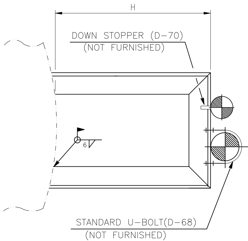
FIG. -B (PLAN VIEW)
