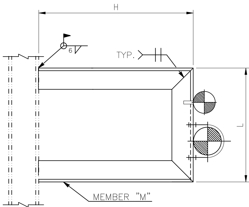
FIG. -A (PLAN VIEW)
