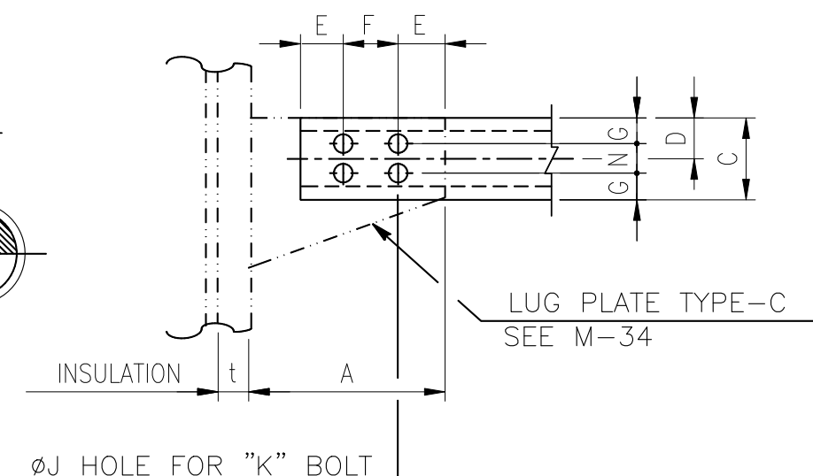
DETAIL "A"
