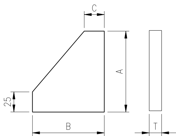
DETAIL "Z"
