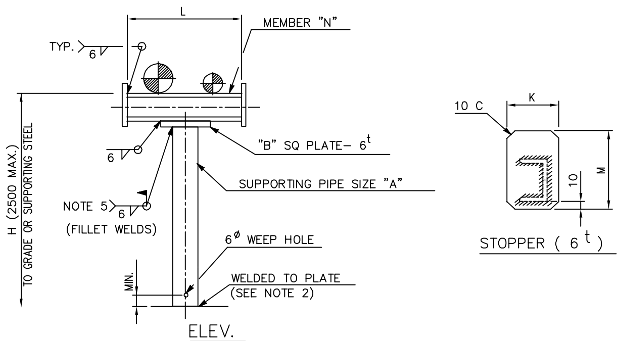
DIMENSIONS (mm)
