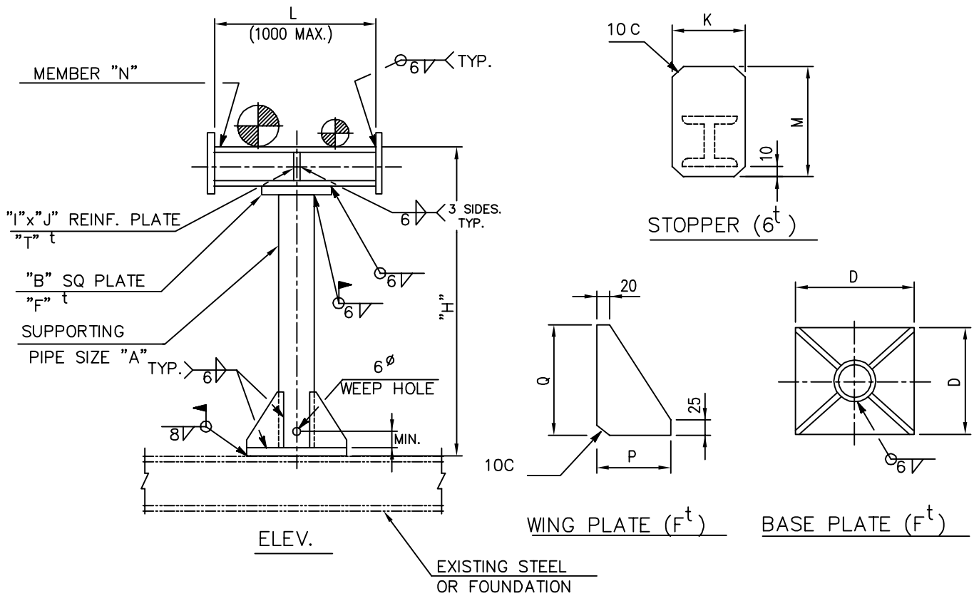
DIMENSIONS (mm)
