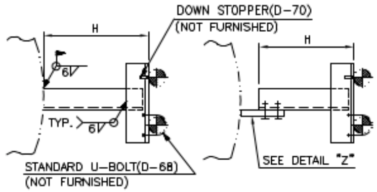
FIG.-B (PLAN VIEW)
