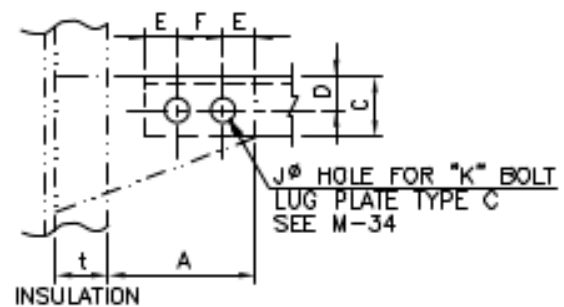
DETAIL "Z"
