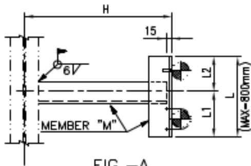
FIG.-A (PLAN VIEW)
