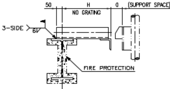
FIG.-A (ELEV. VIEW FOR W/ F. P.)
