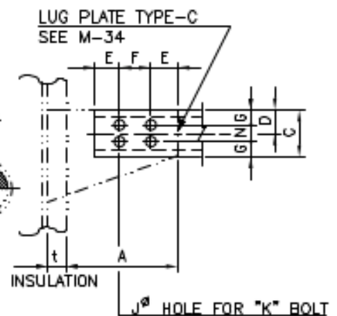
DETAIL "Z"
