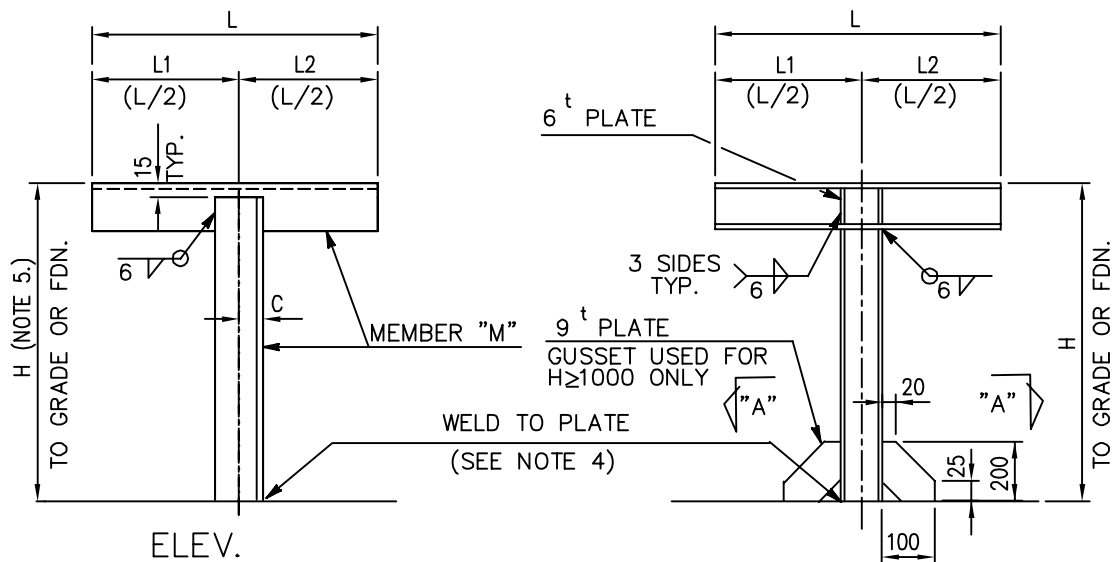
DIMENSION (mm)
