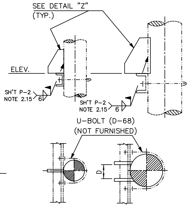
FIG. -B (FOR BARE PIPE)
