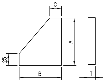
DETAIL "Z"
