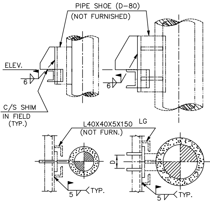
FIG. -A (FOR INS. PIPE)
