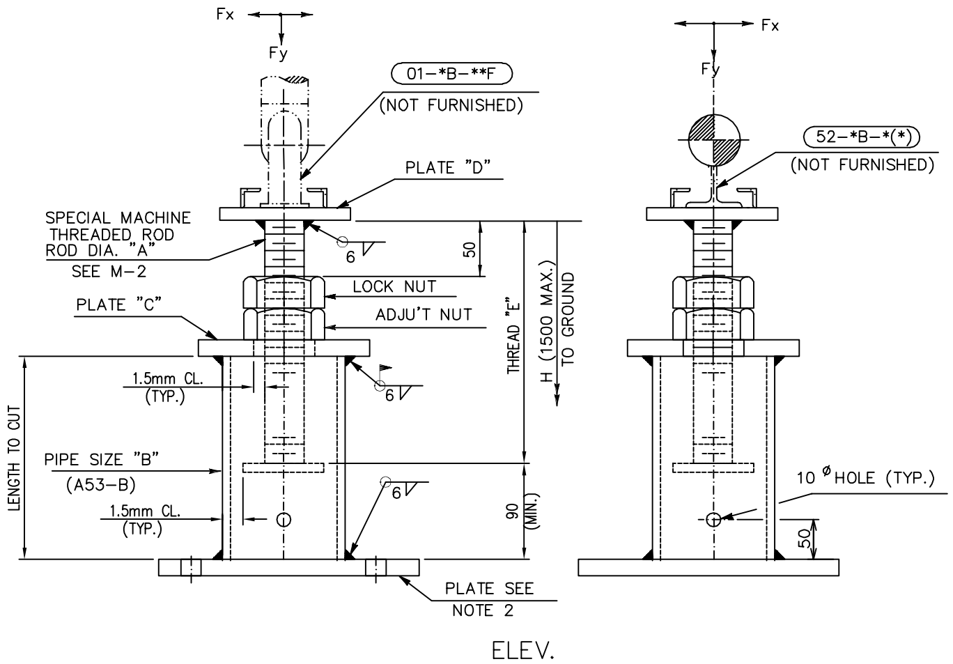
DIMENSIONS (mm)
