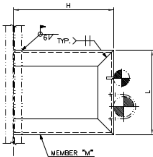
FIG.-A (PLAN VIEW)
