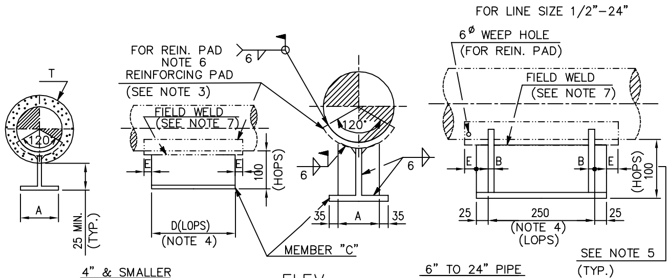
DIMENSION (mm)
