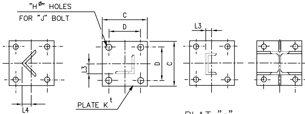
PLATE "c"
