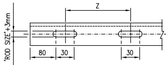
SLOT HOLE DETAIL
