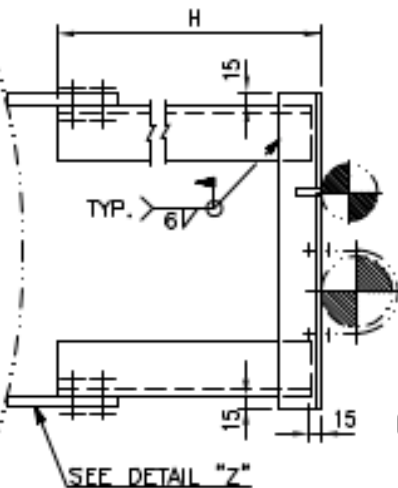
FIG.-C (PLAN VIEW)
