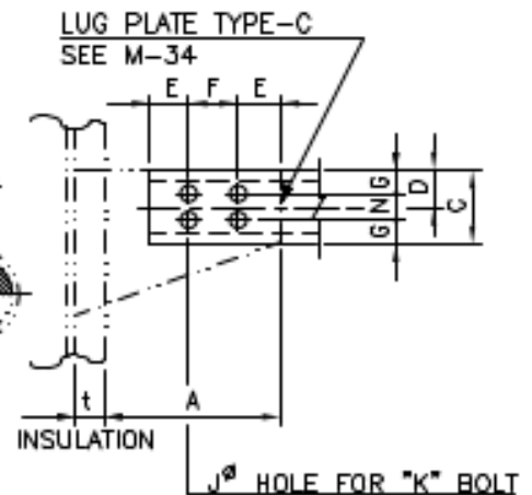
DETAIL "Z"
