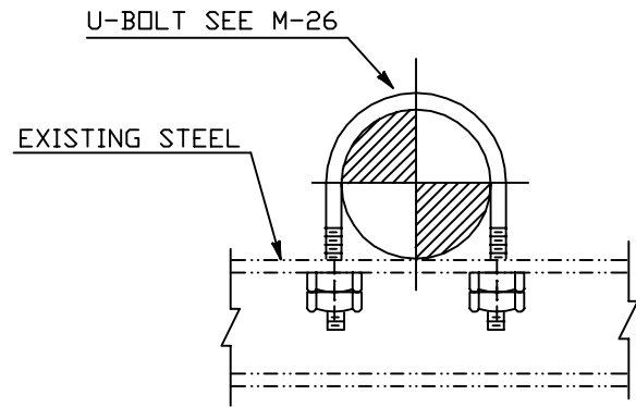
FIG.-B (FIXED)
