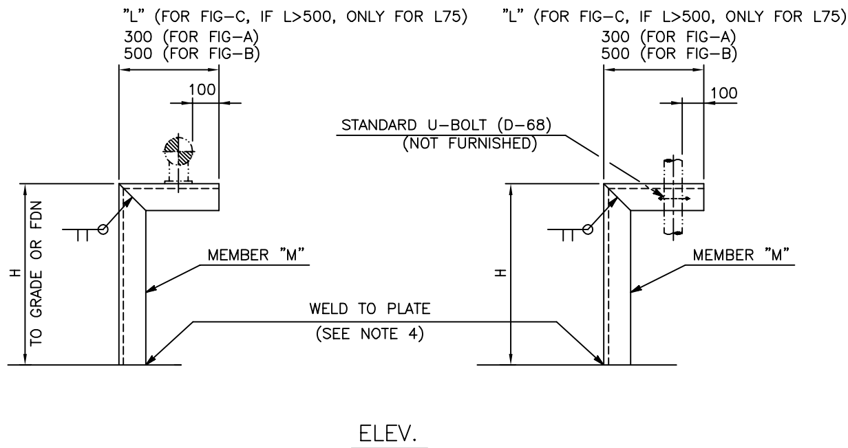
DIMENSIONS (mm)
