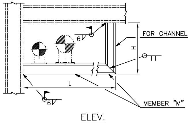
DIMENSIONS (mm)
