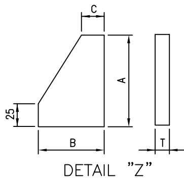
DIMENSIONS (mm)
