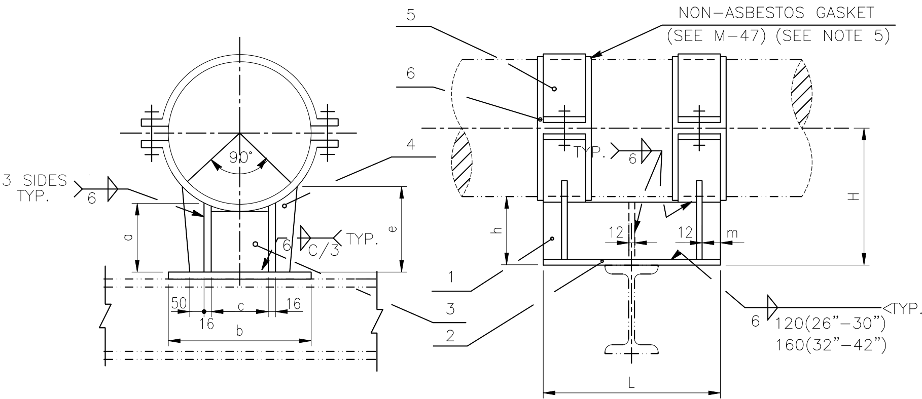
DIMENSIONS (mm)
