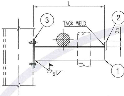
型式：SS13SW
