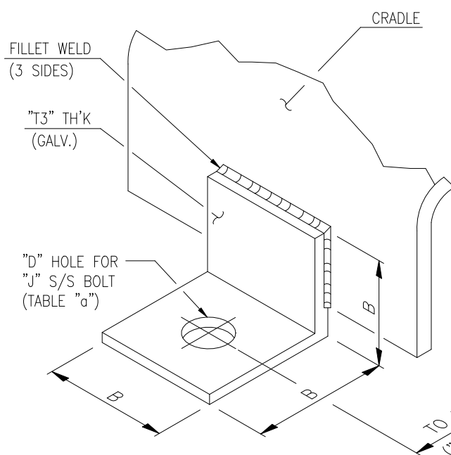
DETAIL "Y"
