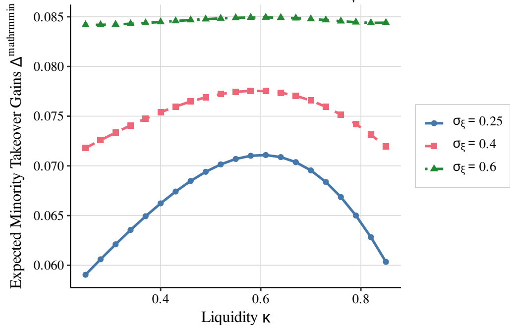
Sensitivity to Bidder Heterogeneity \sigma_\xi
