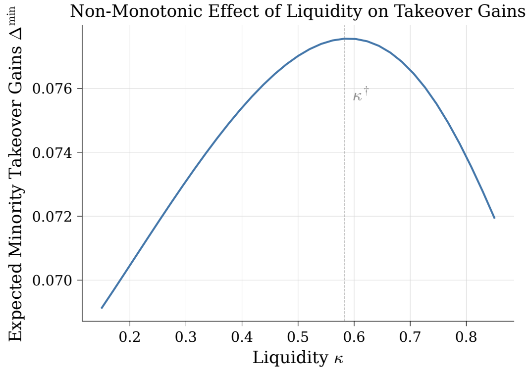
Figure H.2: Nonmonotonic effect of liquidity on expected minority takeover gains. The vertical dashed line marks the turning point \kappa^\dagger (the maximizer of \Delta^{\min} on the plotted grid) in the baseline calibration.
