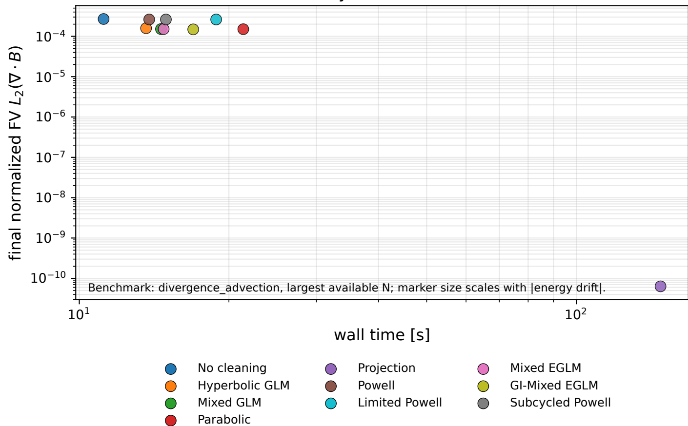
Accuracy-cost Pareto view
