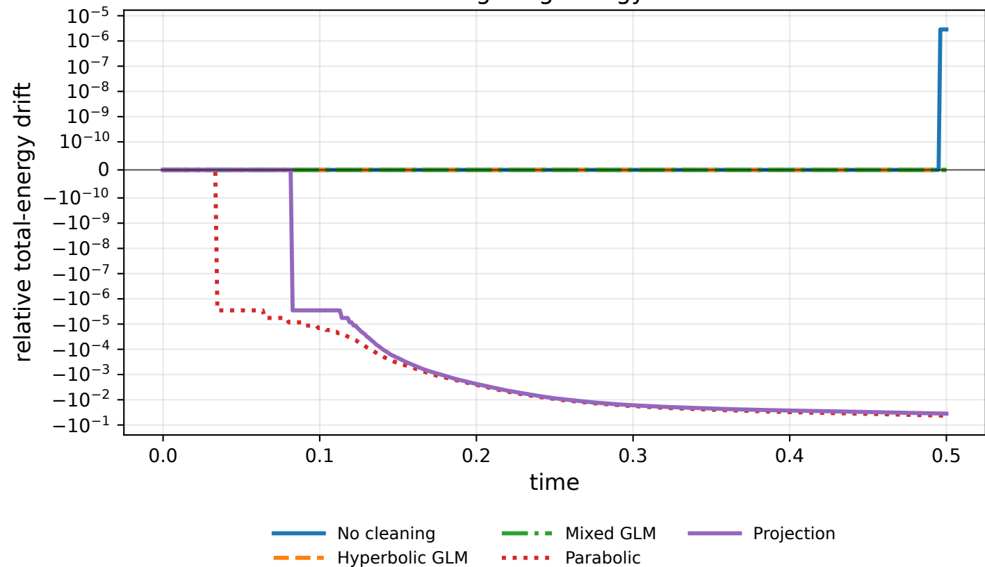
Orszag-Tang energy drift
