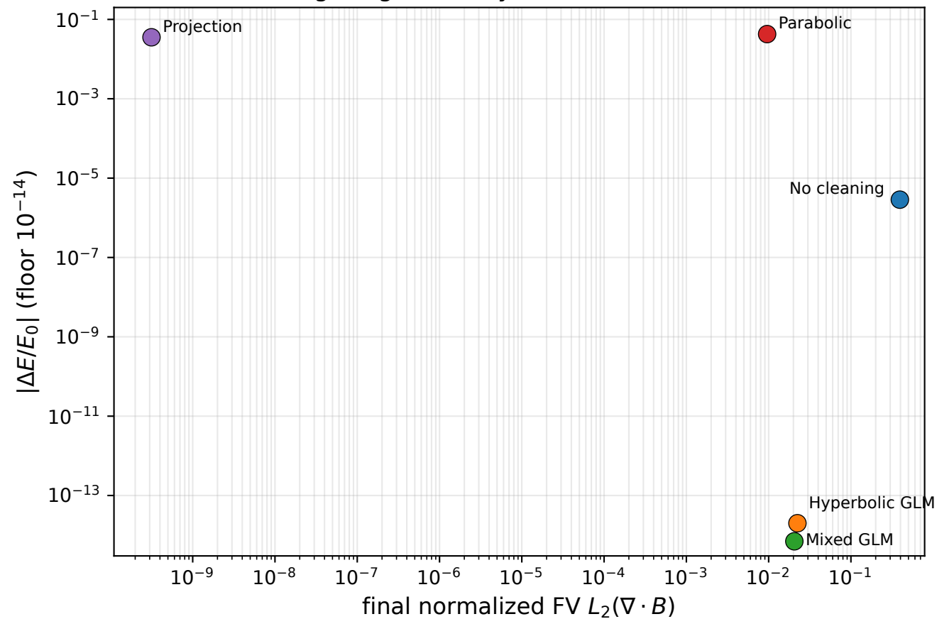
Orszag-Tang accuracy-conservation trade-off
