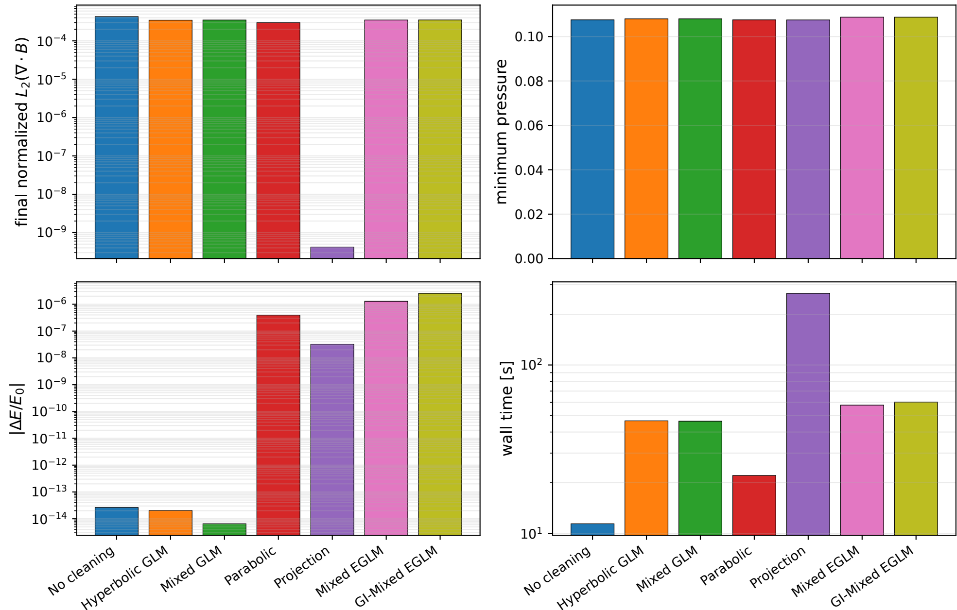
Method scorecard: Orszag-Tang performance benchmark
