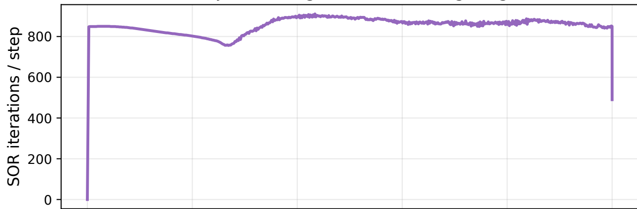
Projection diagnostics on Orszag-Tang
